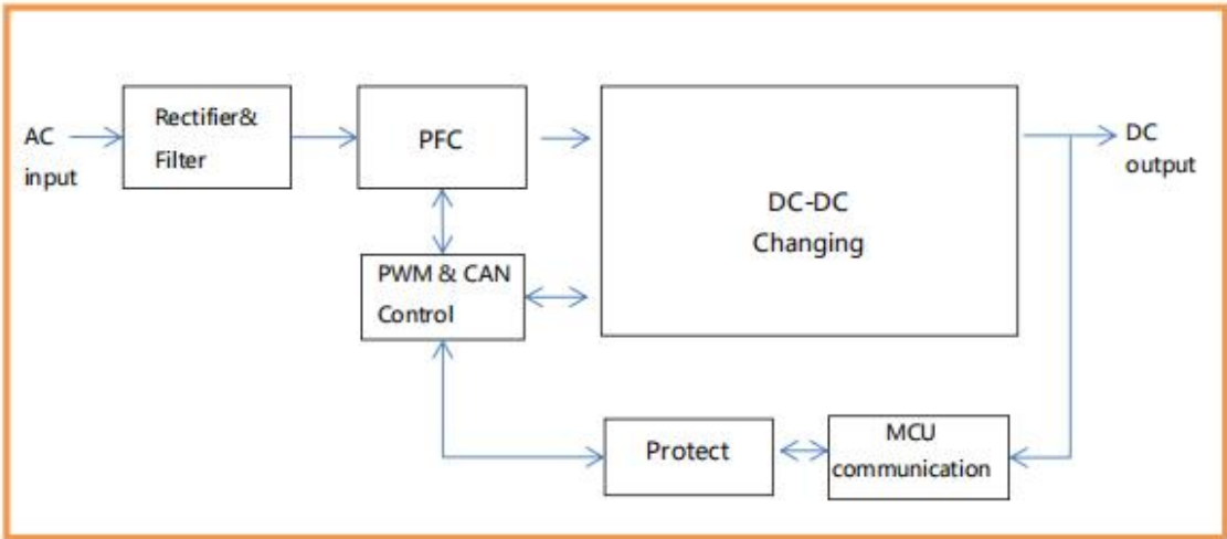
Charging module topology framework
