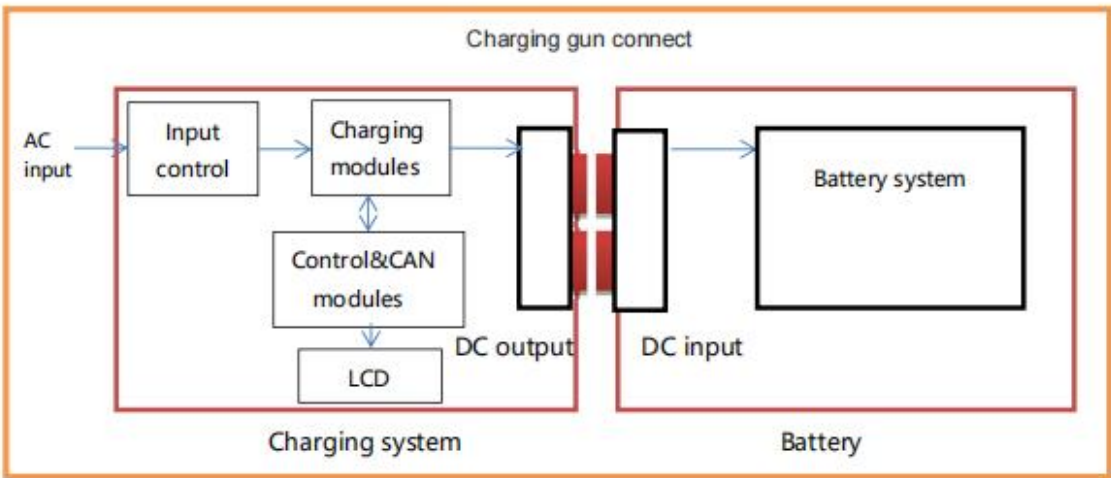
System Architecture
